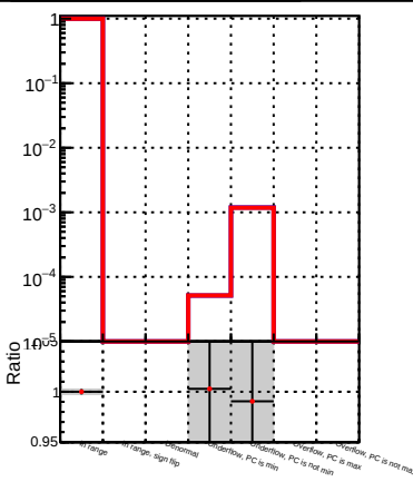
(PacketCandidate::bestTrack() - reco::Track)reco::Track in cov(qoverp, qoverp) status and sign flag
