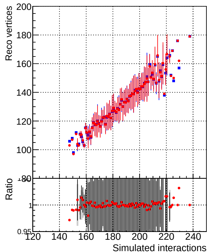
RecoVtx_vs_GenVtx
