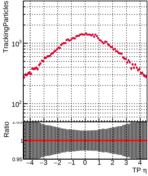
N of simulated tracks vs TP \eta Legend: DQM_beforePR (blue line with squares), DQM_correctCheck (red line with circles)
