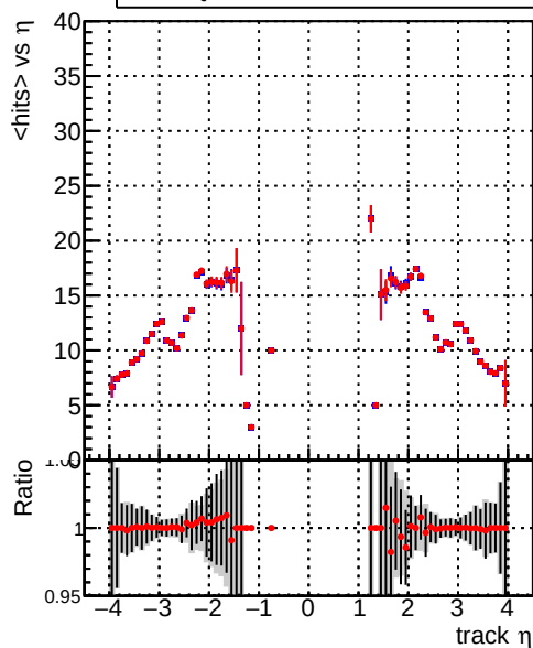
mean hits vs \eta — DQM_beforePR — DQM_correctCheck
