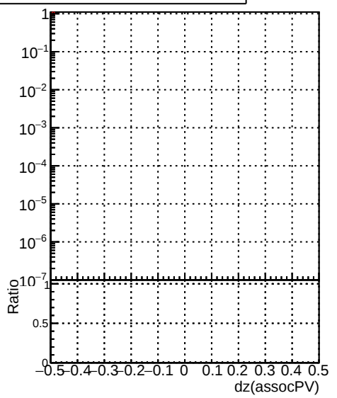
(PackedCandidate::dz(assocPV) - reco::Track::dz(assocPV))/reco::Track with over- and underflow, and sign flip
