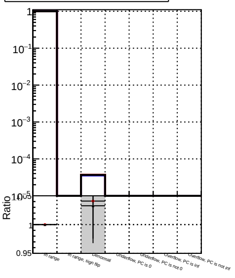
(PackedCandidate::dz(assocPV) - reco::Track::dz(assocPV))/reco::Track status
