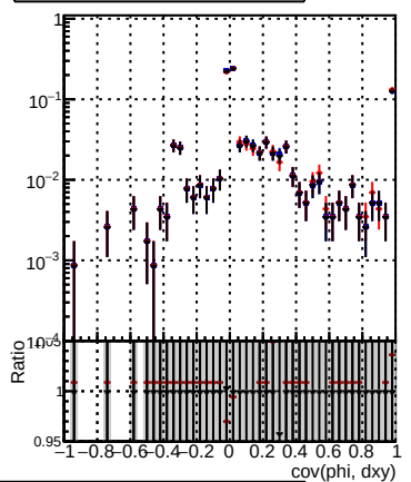
(packedCandidate:bestTrack) - reco:Track|reco:Track in cov(phi, dxy) with over and underflow, and sign flip
