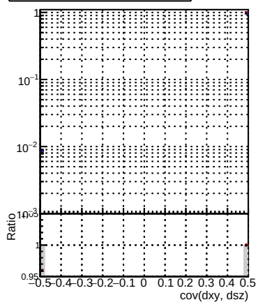
(packedCandidate:bestTrack) - reco:Track|reco:Track in cov(dxy, dsz) with over and underflow, and sign flip
