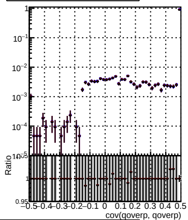
(PacketCandidate::bestTrack() - reco::Track)(reco::Track in cov(goverp, goverp) and underflow and overflow)
