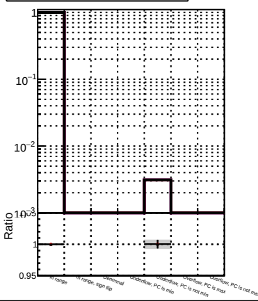
(PacketCandidate::bestTrack() - reco::Track)(reco::Track in cov(goverp, goverp) status)
