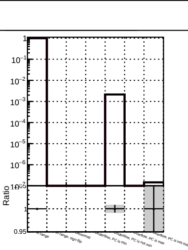
(PacketCandidate::bestTrack() - reco::Track)(reco::Track in cov(lambda, lambda))
