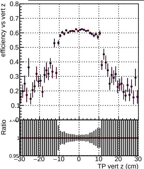
Efficiency vs TP vert z (cm) Legend: DQM_beforePR (blue line with circles) DQM_afterPR (red line with circles) DQM_partialCheck (black line with circles)
