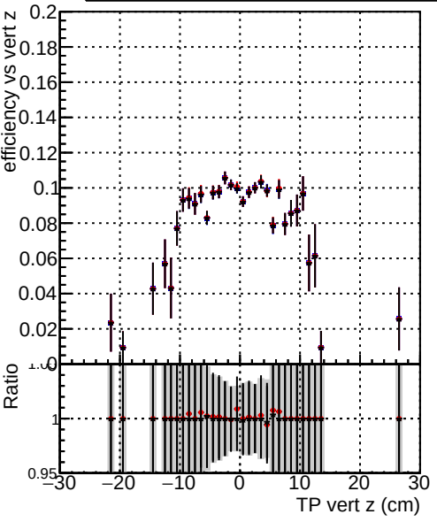
Efficiency vs TP vert z (cm) Legend: DQM_beforePR (blue circles) DQM_afterPR (red circles) DQM_partialCheck (black circles)
