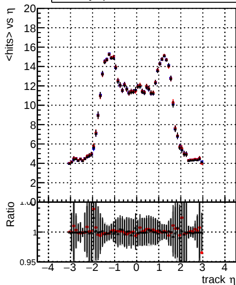
mean hits vs \eta — DQM_beforePR — DQM_afterPR — DQM_partialCheck
