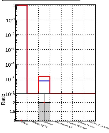
(PackedCandidate::dxy() - reco::Track::dxy(assocPV))/reco::Track status
