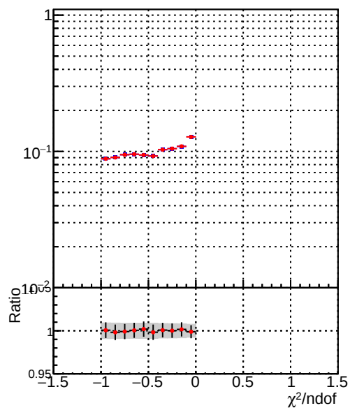
PackedCandidate::bestTrack() - reco::Track in normalizedChi2Q
