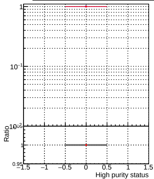
PackedCandidate Legend: DQM_beforePR (blue line with circles) DQM_afterPR (red line with circles)
