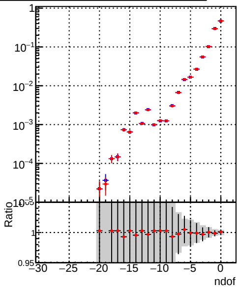
PackedCandidate Legend: DQM_beforePR (blue line with circles) DQM_afterPR (red line with circles)
