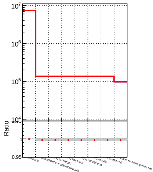
PackedCandidate Legend: DQM_beforePR (blue line with circles) DQM_afterPR (red line with circles)
