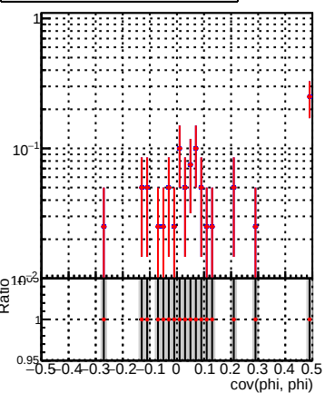
(PacketCandidate::bestTrack() - reco::Track)reco::Track in cov(phi, dsz) and cov(phi, phi)
