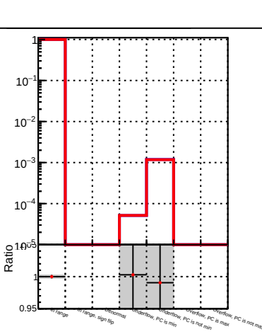
(PacketCandidate::bestTrack() - reco::Track)reco::Track in cov(lambda, lambda) status
