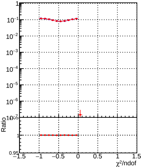
PackedCandidate::bestTrack() - reco::Track in normalizedChi2()
