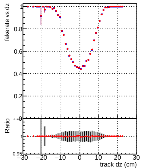
—●— DQM_beforePR —●— DQM_afterPR
