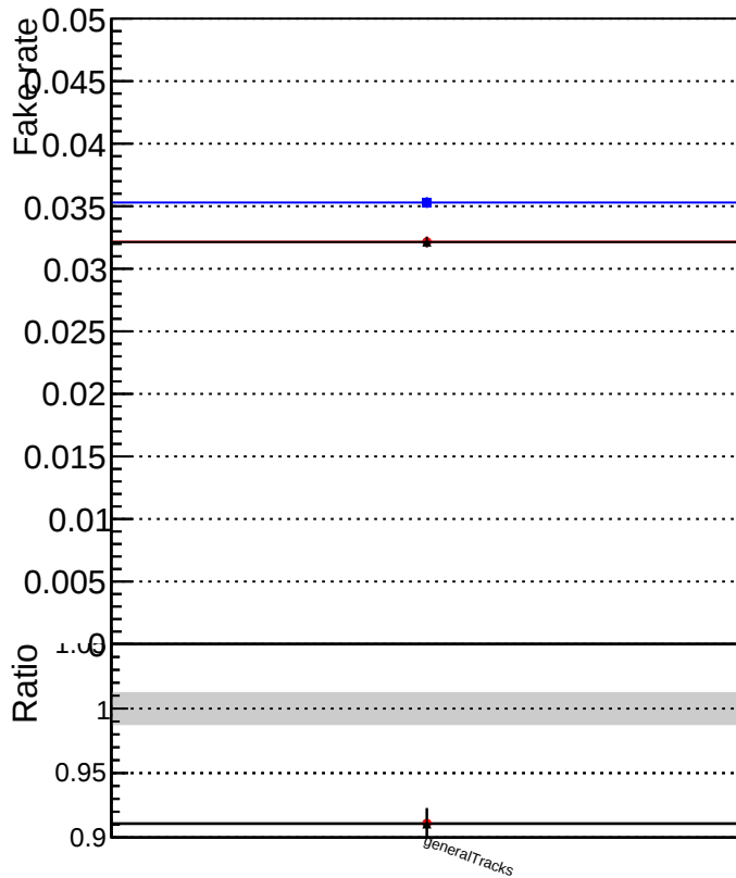
Fakerate vs collection
