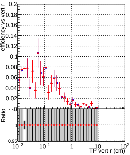
Efficiency vs TP vert r (cm) Legend: DQM_beforePR (blue line with squares), DQM_afterPR (red line with circles)
