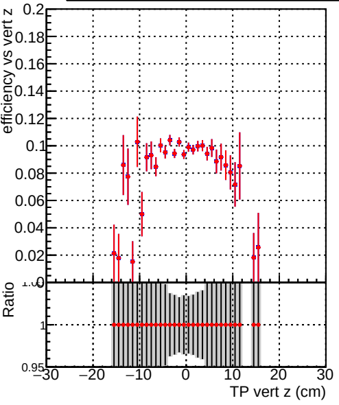
Efficiency vs TP vert z (cm) Legend: DQM_beforePR (blue line with squares), DQM_afterPR (red line with circles)
