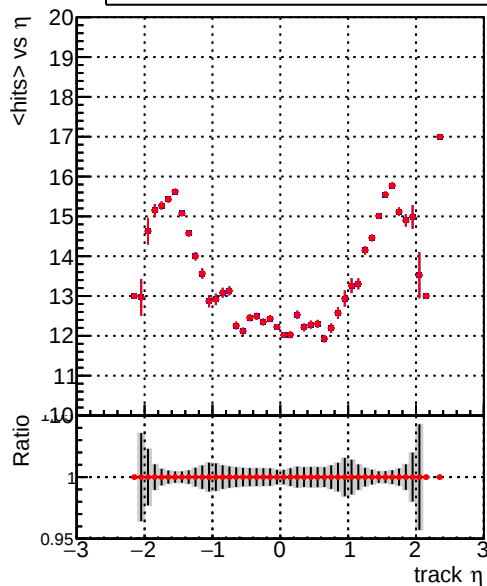
mean hit — DQM_beforePR — DQM_afterPR
