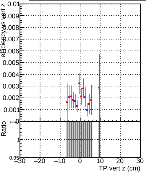
Efficiency vs TP vert z (cm) DQM_beforePR (blue line with dots) DQM_afterPR (red line with dots)
