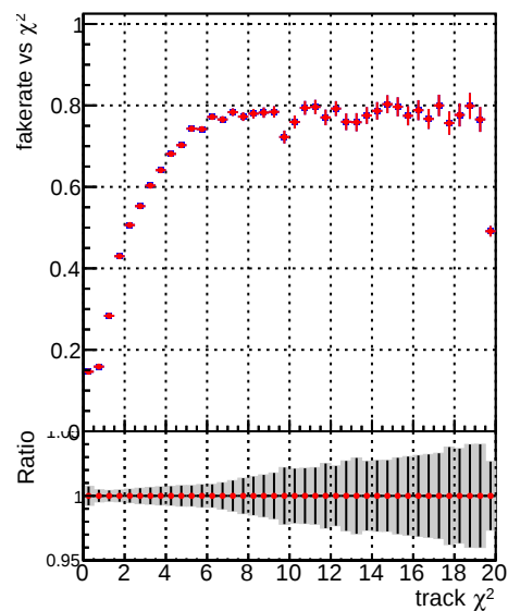
Fake rate vs. DQM_beforePR DQM_afterPR
