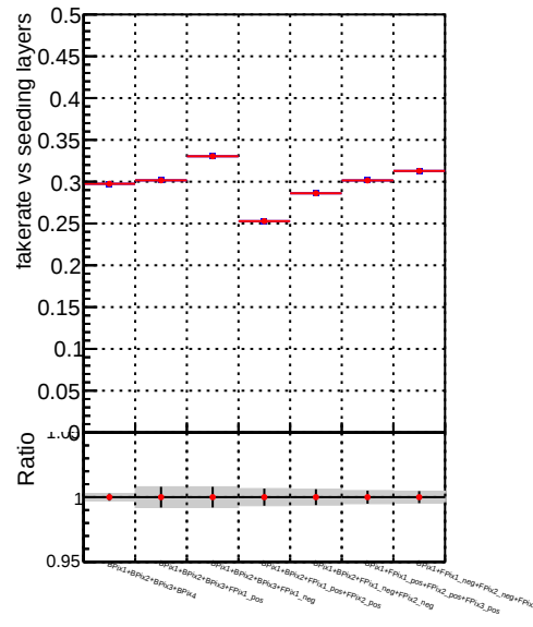
Fake rate vs. DQM_beforePR DQM_afterPR
