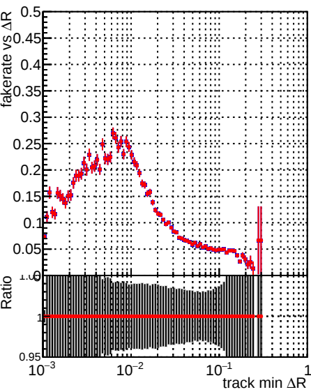
Fake rate vs \Delta R(\text{track, jet}) Legend: \blacksquare DQM_beforePR \bullet DQM_afterPR
