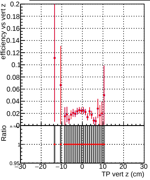
Efficiency vs vert z Legend: DQM_beforePR (blue line with dots), DQM_afterPR (red line with dots)
