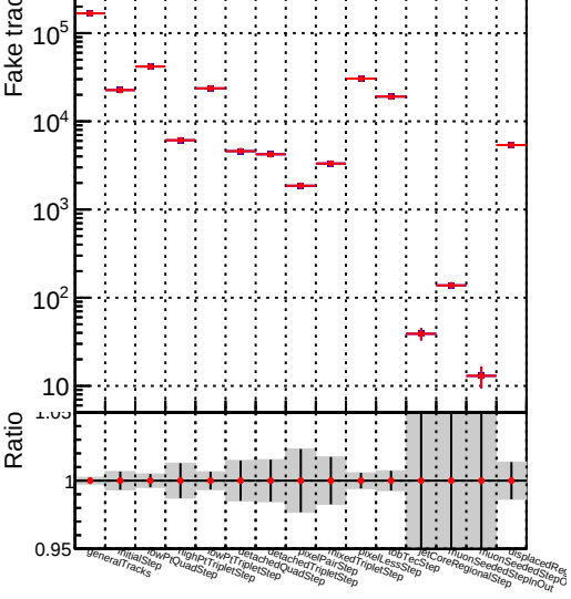
Number of fake tracks vs collection
