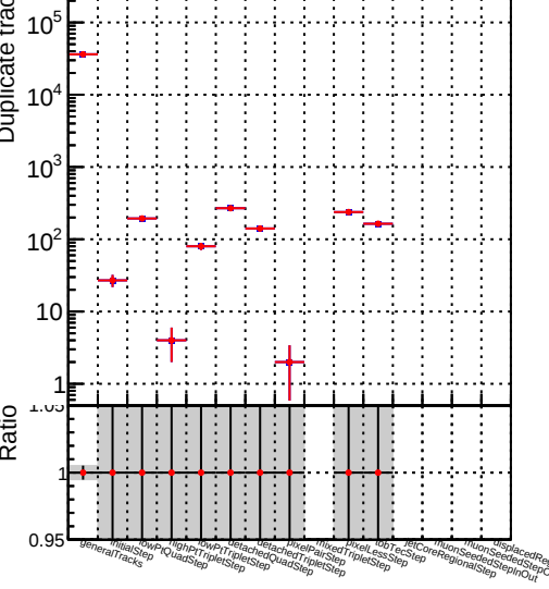
Number of duplicate tracks vs collection
