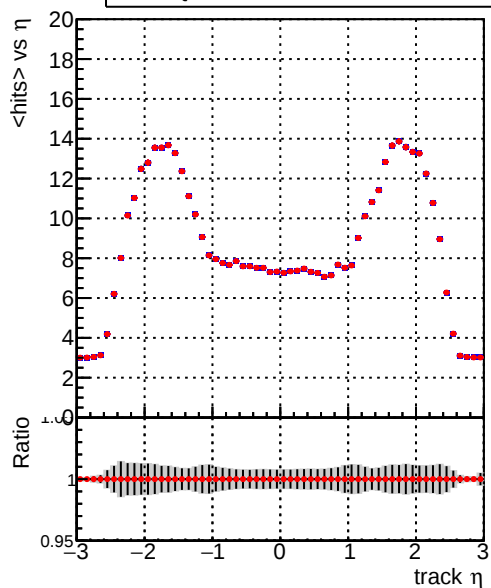
mean hits vs \eta — DQM_beforePR — DQM_afterPR
