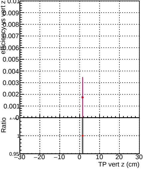
Efficiency vs vert z Legend: DQM_correctCheck_mu_pt1to1000_eta2p5to4p0 (blue line with dots) DQM_original_mu_pt1to1000_eta2p5to4p0 (red line with dots)
