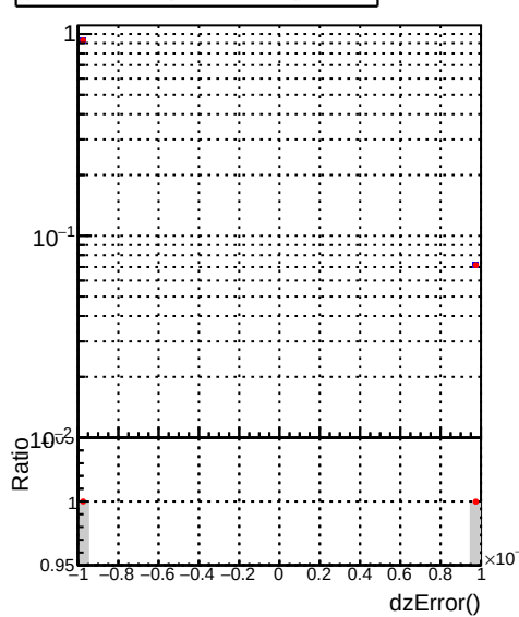
(PackedCandidate::dxyError() - reco::Track::dxyError())/reco::Track with over- and underflow, and sign flip
