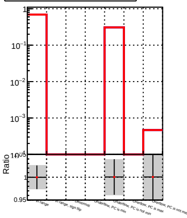
(PackedCandidate::bestTrackQ - reco::Track)reco::Track in cov(phi, phi) status
