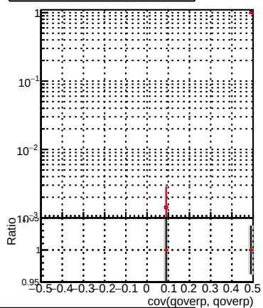
(PackedCandidate::bestTrackQ - reco::Track)reco::Track in cov(qoverp, qoverp) status
