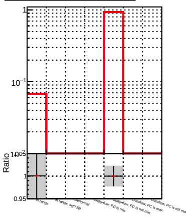
(PackedCandidate::bestTrackQ - reco::Track)reco::Track in cov(lambda, dsz) status
