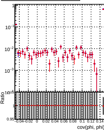
(PackedCandidate::bestTrackQ - reco::Track)reco::Track in cov(phi, phi)
