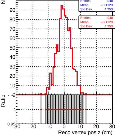
Recons DQM_correctCheck_mu_pt1to1000_eta2p5to4p0 DQM_original_mu_pt1to1000_eta2p5to4p0
