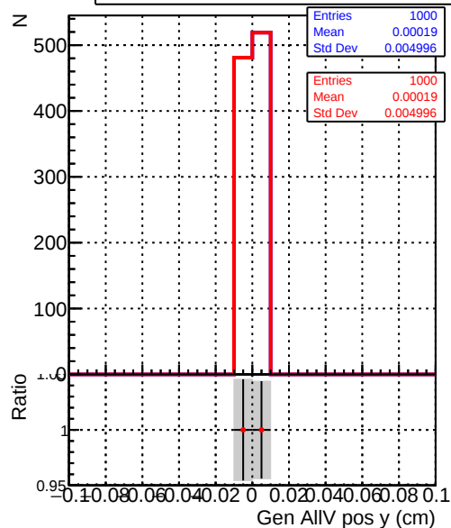
Legend: DQM_correctCheck_mu_pt1to1000_eta2p5to4p0 (Blue line with markers) DQM_original_mu_pt1to1000_eta2p5to4p0 (Red line with markers)
