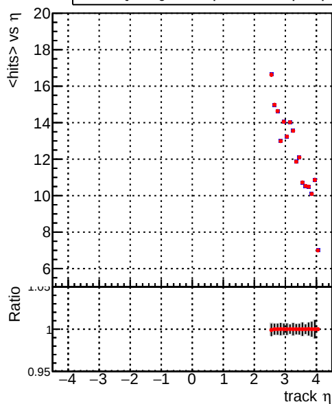
— DQM_correctCheck_mu_pt1to1000_eta2p5to4p0 — DQM_original_mu_pt1to1000_eta2p5to4p0
