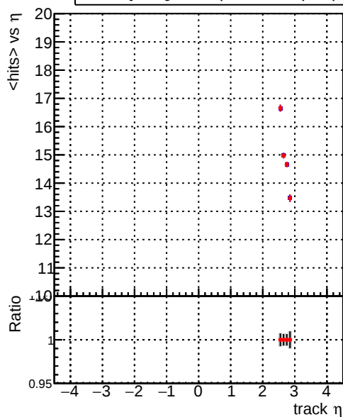
mean hits — DQM_correctCheck_mu_pt1to1000_eta2p5to4p0 — DQM_original_mu_pt1to1000_eta2p5to4p0
