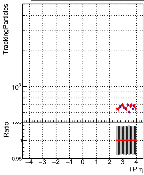
Legend: DQM_correctCheck_mu_pt1to1000_eta2p5to4p0 (blue line), DQM_original_mu_pt1to1000_eta2p5to4p0 (red line)
