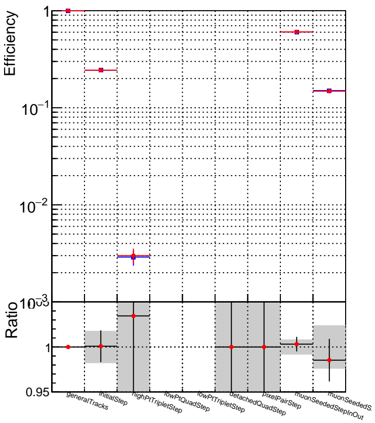
■ DQM_correctCheck_mu_pt1to1000_eta2p0to2p5 ■ DQM_original_mu_pt1to1000_eta2p0to2p5
