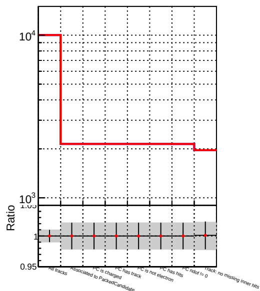
PackedCandidate DQM_correctCheck_mu_pt1to1000_eta2p0to2p5 DQM_original_mu_pt1to1000_eta2p0to2p5
