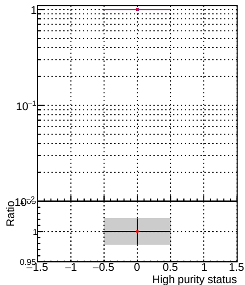
PackedCandidate DQM_correctCheck_mu_pt1to1000_eta2p0to2p5 DQM_original_mu_pt1to1000_eta2p0to2p5
