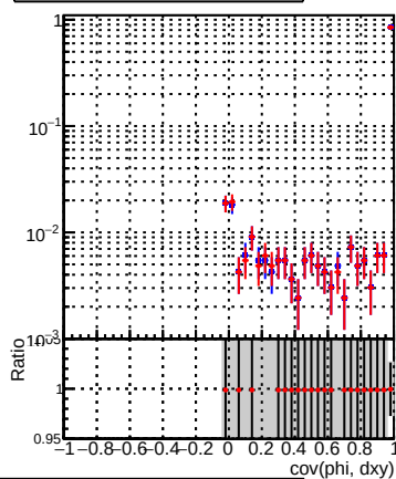
DQM_correctCheck_mu_pt1to1000_eta2p0to2p5 DQM_original_mu_pt1to1000_eta2p0to2p5
