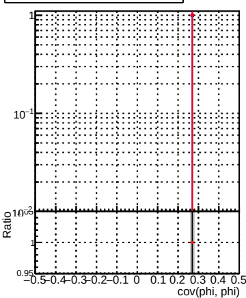
(PackedCandidate::bestTrack() - reco::Track)reco::Track in cov(phi, phi) status
