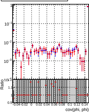
(PackedCandidate::bestTrack() - reco::Track)reco::Track in cov(phi, phi) status
