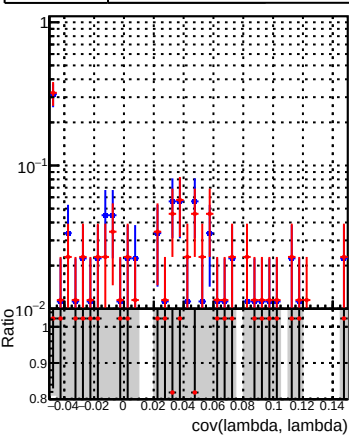
(PackedCandidate::bestTrack() - reco::Track)reco::Track in cov(lambda, lambda) status
