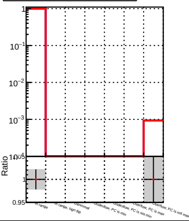
(PackedCandidate::bestTrack() - reco::Track)reco::Track in cov(lambda, lambda) status
