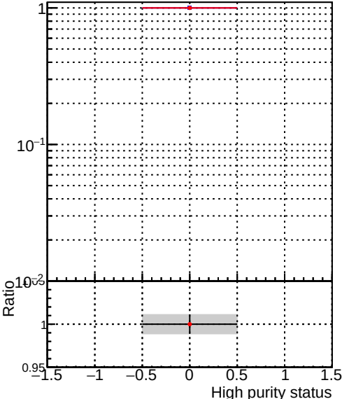
PackedCandidate DQM_correctCheck_mu_pt1to1000_eta2p0to2p5 DQM_original_mu_pt1to1000_eta2p0to2p5
