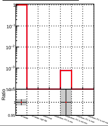
(PackedCandidate::bestTrack() - reco::Track)reco::Track in cov(goverp, goverp) status
