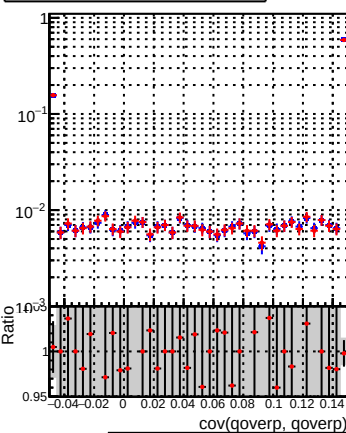
(PackedCandidate::bestTrack() - reco::Track)reco::Track in cov(goverp, goverp)
