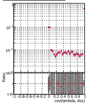
(PackedCandidate::bestTrack() - reco::Track)reco::Track in cov(lambda, dsz) not max and not min
