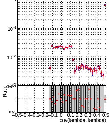
(PackedCandidate::bestTrack() - reco::Track)reco::Track in cov(lambda, lambda) not max and not min
