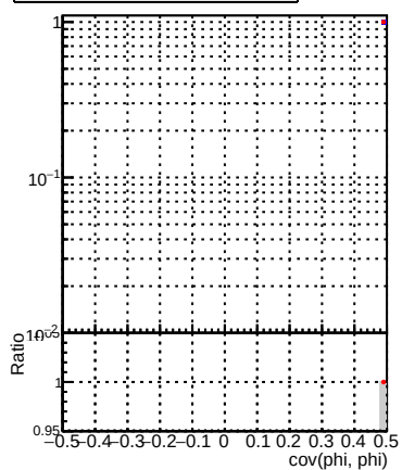
(PackedCandidate::bestTrack() - reco::Track)reco::Track in cov(phi, phi) not max and not min
