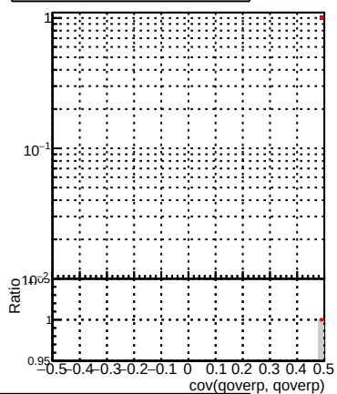
(PackedCandidate::bestTrack() - reco::Track)reco::Track in cov(goverp, goverp) not max and not min
