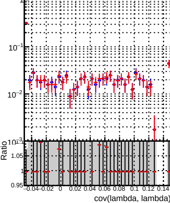
(PackedCandidate::bestTrack() - reco::Track)reco::Track in cov(lambda, lambda)
