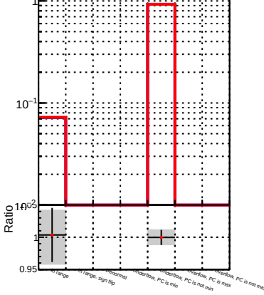
(PackedCandidate::bestTrack() - reco::Track)reco::Track in cov(lambda, lambda) status
