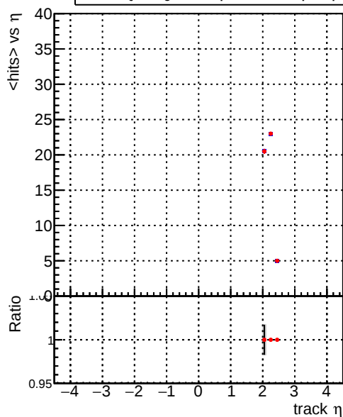
mean hits vs \eta — DQM_correctCheck_mu_pt1to1000_eta2p0to2p5 — DQM_original_mu_pt1to1000_eta2p0to2p5
