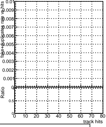
■ DQM_correctCheck_mu_pt1to1000_eta2p0to2p5 ■ DQM_original_mu_pt1to1000_eta2p0to2p5
