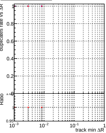
Legend: DQM_correctCheck_mu_pt1to1000_eta2p0to2p5 (blue line with dots) DQM_original_mu_pt1to1000_eta2p0to2p5 (red line with dots)
