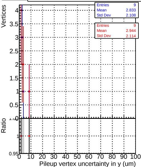
Legend: DQM_correctCheck_mu_pt1to1000_eta2p0to2p5 (blue line with dots), DQM_original_mu_pt1to1000_eta2p0to2p5 (red line with dots)
