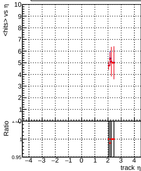
— DQM_correctCheck_mu_pt1to1000_eta2p0to2p5 — DQM_original_mu_pt1to1000_eta2p0to2p5
