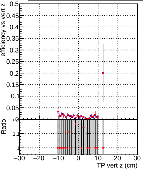
Efficiency vs vert z Legend: — DQM_correctCheck_mu_pt1to1000_eta2p0to2p5 — DQM_original_mu_pt1to1000_eta2p0to2p5
