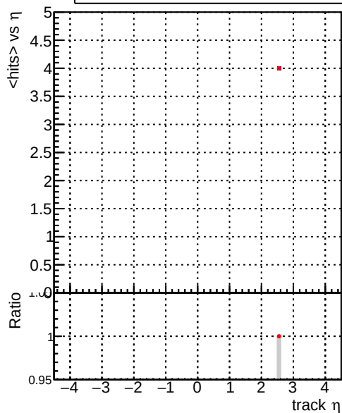
mean hits — DQM_correctCheck_mu_pt1to1000_eta2p0to2p5 — DQM_original_mu_pt1to1000_eta2p0to2p5
