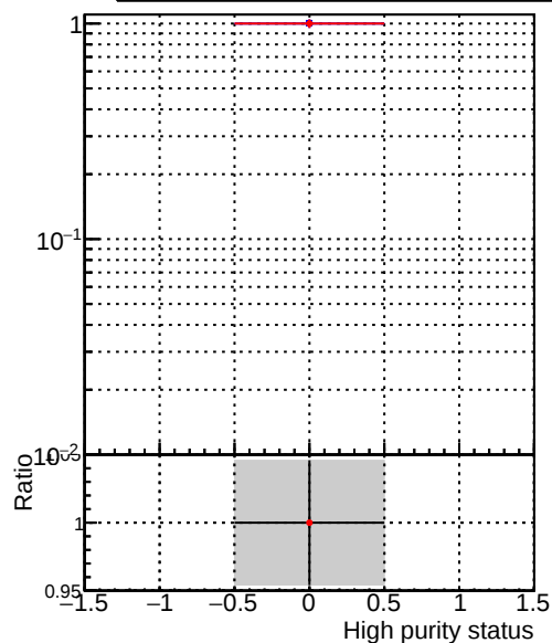
PackedCandidate DQM_correctCheck_mu_pt1to1000_eta1p5to2p0 DQM_original_mu_pt1to1000_eta1p5to2p0
