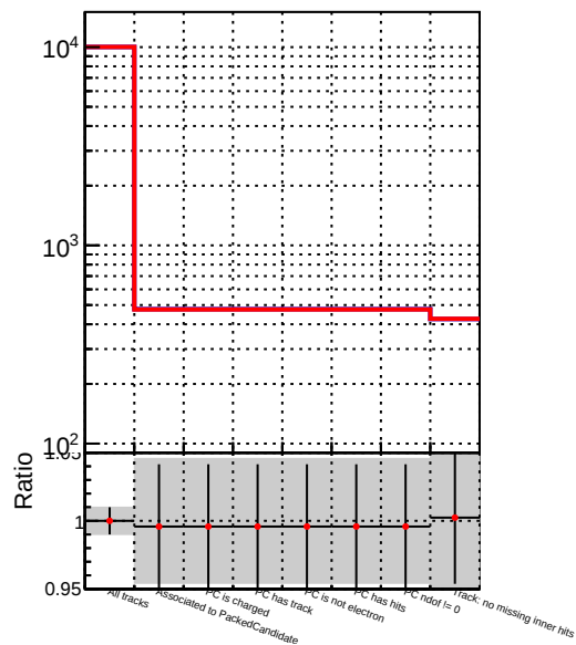
PackedCandidate DQM_correctCheck_mu_pt1to1000_eta1p5to2p0 DQM_original_mu_pt1to1000_eta1p5to2p0
