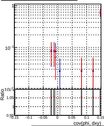
(packedCandidate:bestTrack) - reco:Track(reco:Track in cov(phi, dxy))
