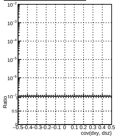
(packedCandidate:bestTrack) - reco:Track(reco:Track in cov(dxy, dsz) status with over and underflow, and sign flip)
