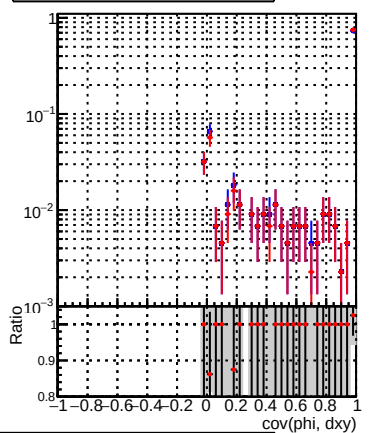
(packedCandidate:bestTrack) - reco:Track(reco:Track in cov(phi, dxy) status with over and underflow, and sign flip)
