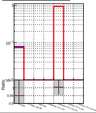
(packedCandidate:bestTrack) - reco:Track(reco:Track in cov(phi, dxy) status)
