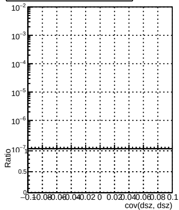
(packedCandidate:bestTrack) - reco:Track(reco:Track in cov(dsz, dsz) status with over and underflow, and sign flip)
