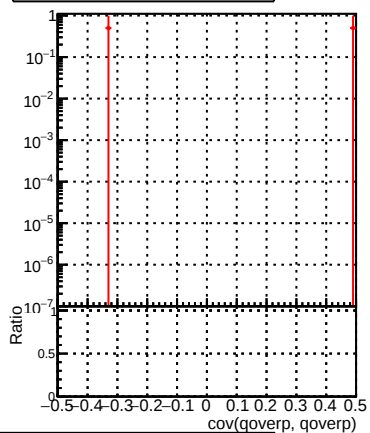
Legend: DQM_correctCheck_mu_pt1to1000_eta1p5to2p0 (blue circles), DQM_original_mu_pt1to1000_eta1p5to2p0 (red line)
