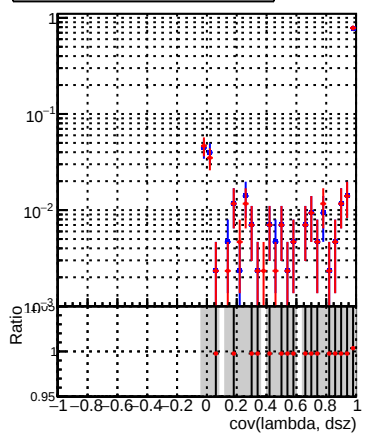
(PackedCandidate::bestTrack() - reco::Track)(reco::Track in cov(lambda, dsz) and not overflow and sign fix)
