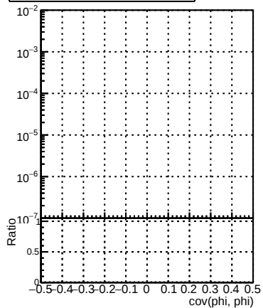
(PackedCandidate::bestTrack() - reco::Track)(reco::Track in cov(phi, phi) and not overflow and sign fix)
