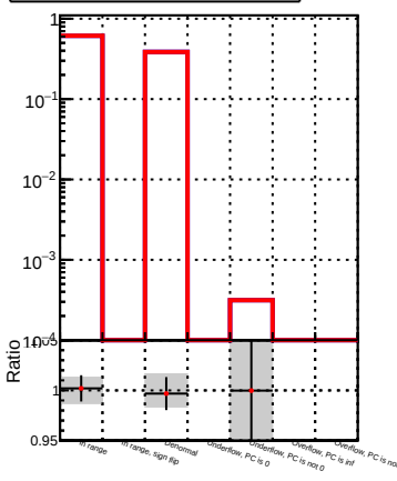
(PacketCandidate::bestTrack() - reco::Track)reco::Track in cov(dxy, dsz) status
