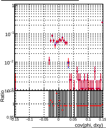
DQM_correctCheck_mu_pt1to1000_eta1p5to2p0 DQM_original_mu_pt1to1000_eta1p5to2p0
